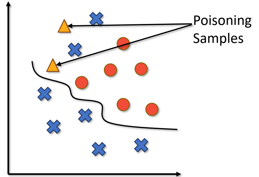
Poisoned Dataset
