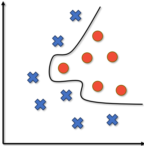
Normal Dataset
